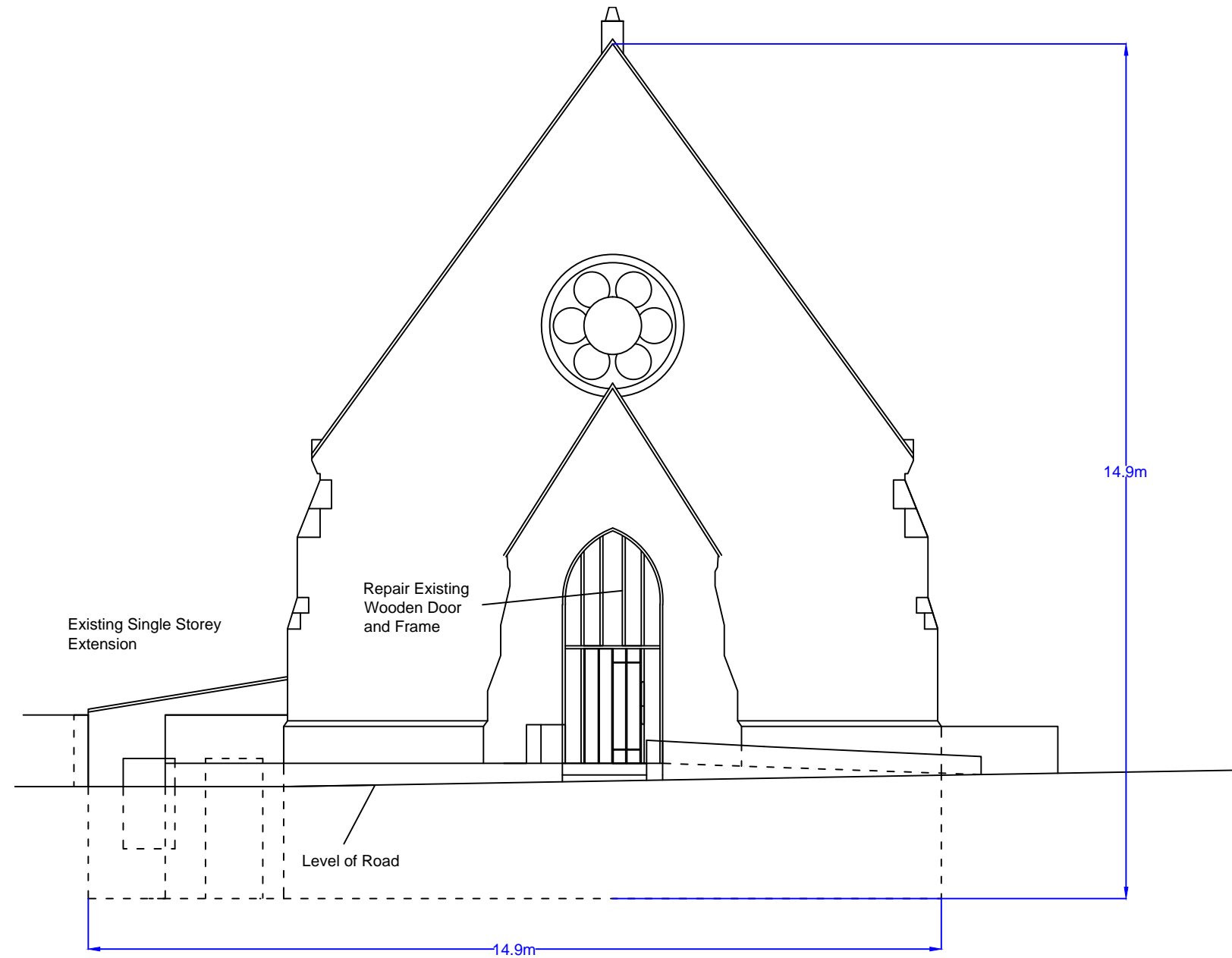
8DT4: 8 Derby Terrace North Elevation As Proposed Page 1 of 1, Scale 1:100 at A3
